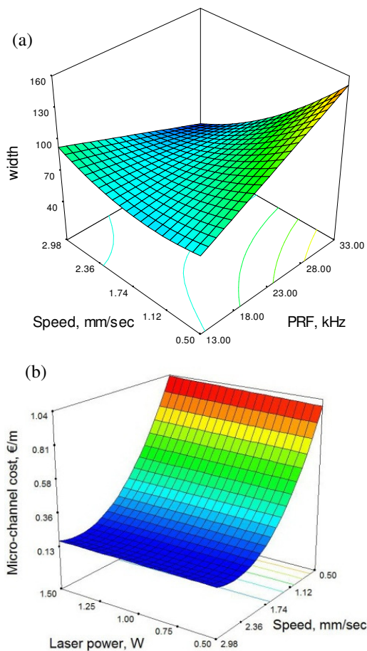
Figure 1: Interactive effect (a) on width value for U and PRF with P = 1 W and (b) on micro-machining cost for P and U with PRF = 23 kHz.
