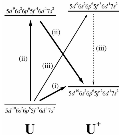
FIG. 5. Direct and indirect paths to the U^+ 5d^{10}6s^26p^65f^26d7s^2 final state following photoexcitation: (i) direct 5f photoionization; (ii) 5d \rightarrow 5f excitation followed by SCK decay; (iii) 5d ionization followed by radiative decay.
