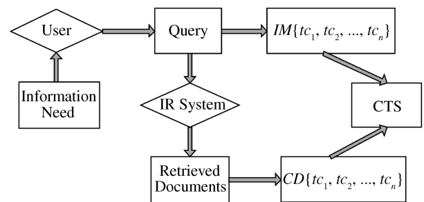
Fig.2. Covering topic score calculation.
