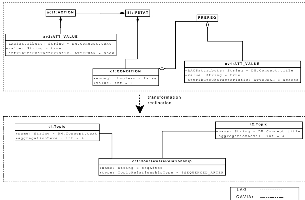
Figure 5: Transformation of LAG model to CAVIAR courseware model
