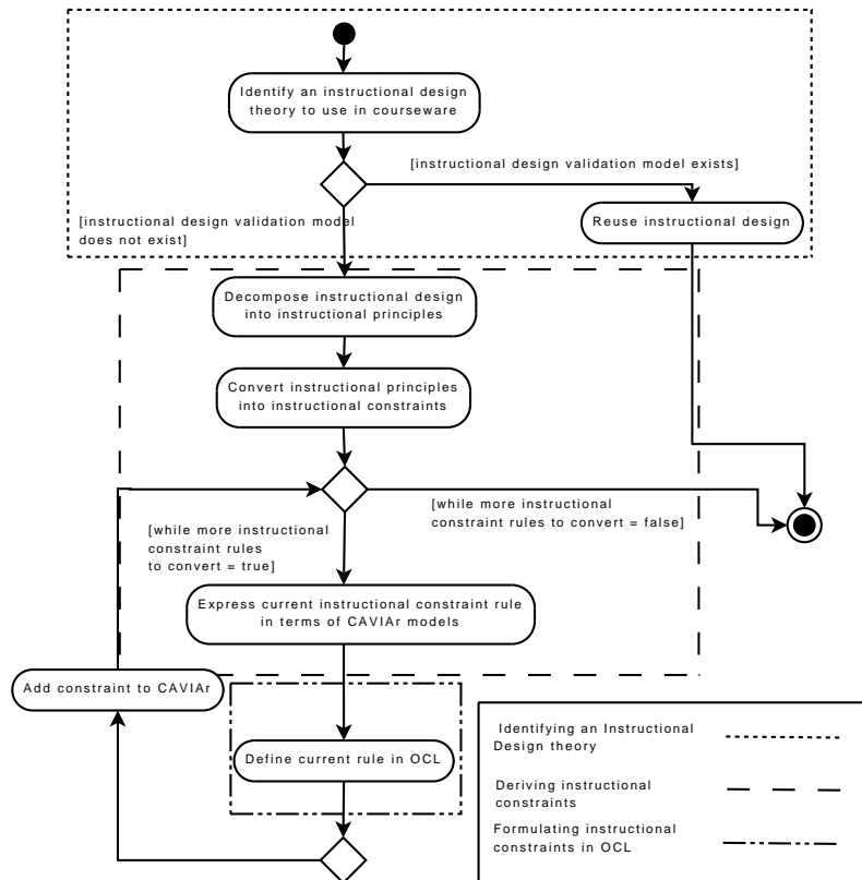
Figure 6: UML Activity Diagram detailing the definition of the CAVIAR Validation Model
