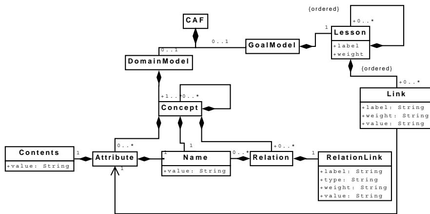
Figure 3: CAF Metamodel defined using ECore
