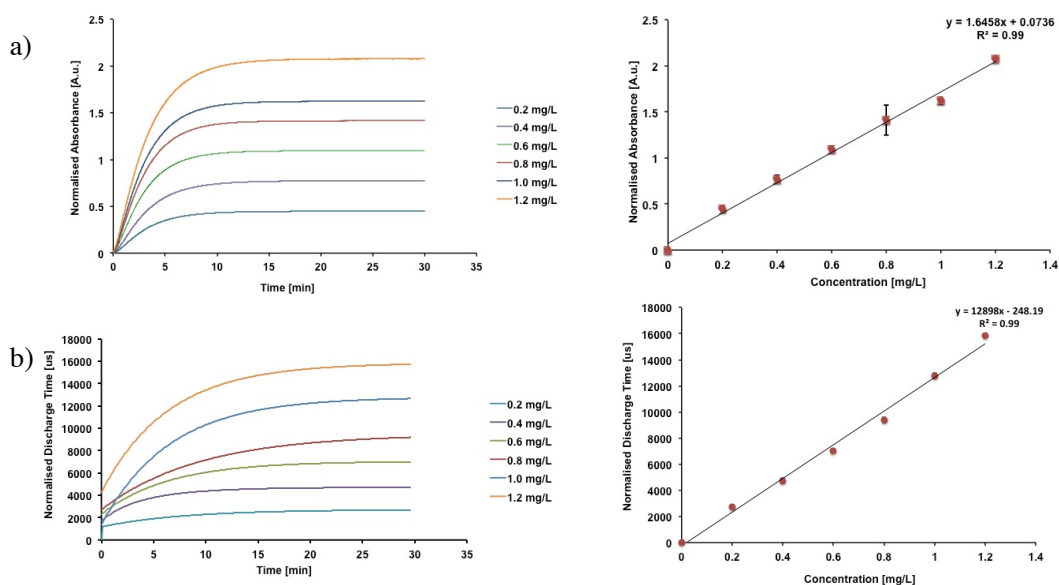
Figure 5: Kinetic study of the colour formation between \text{NO}_2^- and Griess reagent ( n = 2 ) (left side) and absorbance versus nitrite Griess reagent complex concentration (right side) using a UV-Vis spectrometer (a) and the CMAS system (b).
