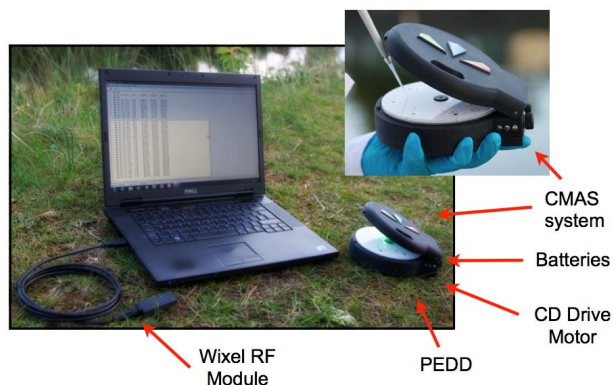
Figure 3: Portable centrifugal microfluidic analysis system.
