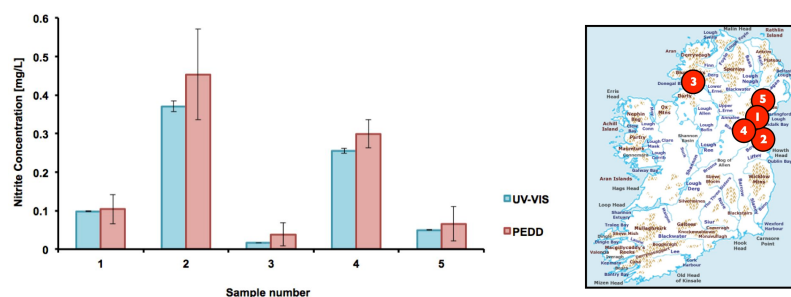
Figure 6: Water nitrite analysis using a bench-top UV-VIS spectrometer and the CMAS device and a map of the sampling places ( n = 3 ).
