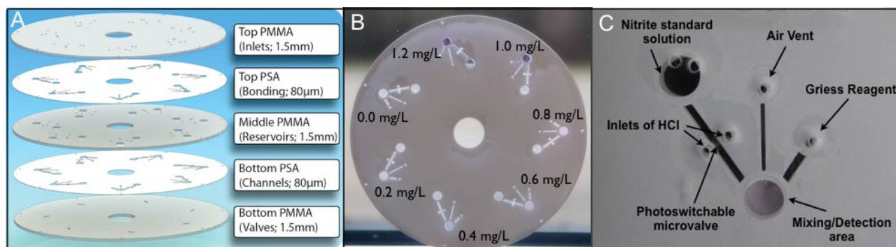
Figure 1: a) Scheme showing the assembly of the micro-fluidic CD, b) picture of the Lab-on-a-Disc and channel consisting of seven microfluidic systems and c) magnification of a single microfluidic system consisting of three chambers.
