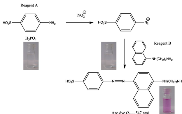
Figure 4: Mechanism of the nitrite detection employing the Griess reaction method [3].
