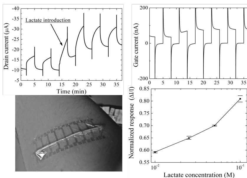
Fig 3: (a) Drain current vs. time (b) Corresponding Gate current vs. Time (c) Conformal OECT with gel shown on forearm (d) Normalized response of the OECT vs. lactate concentration
