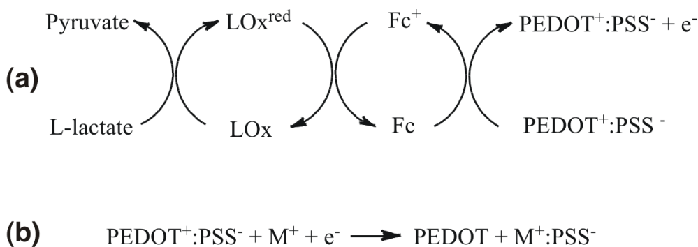
Fig 2: Reactions at the gate electrode (a) and at the channel (b) of the OECT
