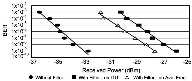
Fig. 4. BER versus received optical power.
