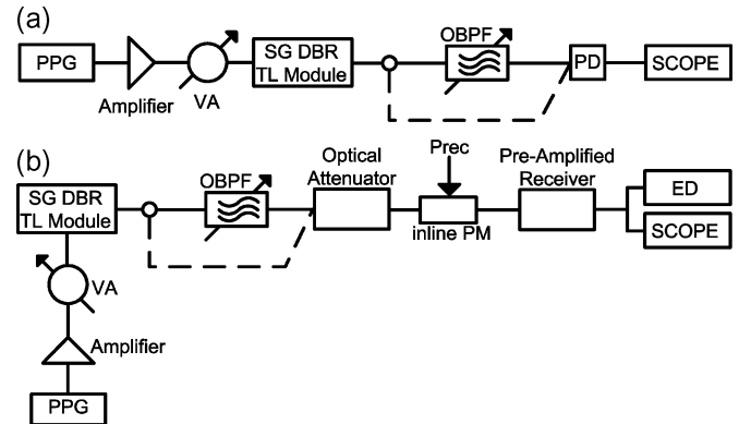
Fig. 1. Experimental setup.
