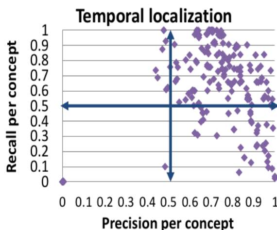
Fig. 14 2015: temporal precision and recall per concept for all teams
