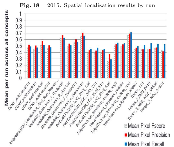
Fig. 18 2015: Spatial localization results by run
