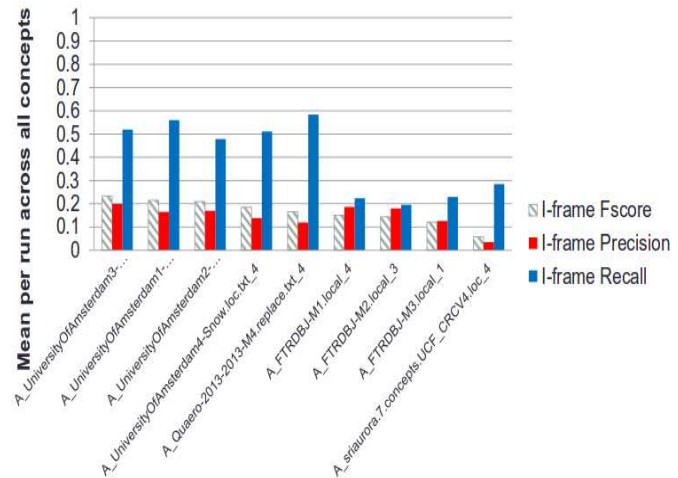
Fig. 11 2013: Temporal localization results by run
