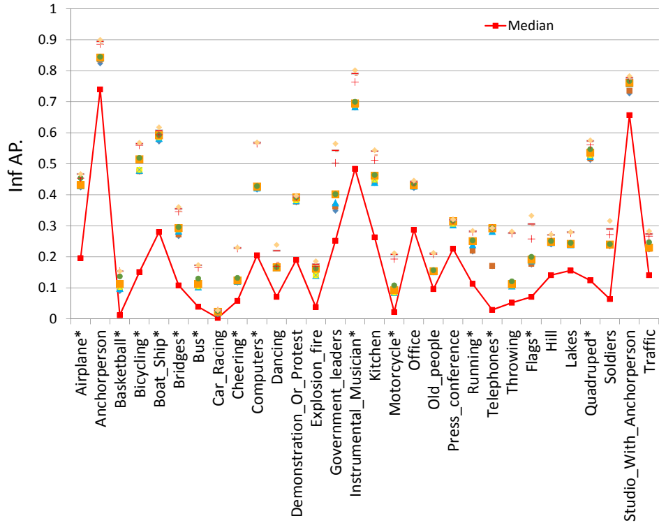
Fig. 7 Top 10 InfAP scores by concept for the 2015 main task. Starred concepts were common between the 2014 and 2015 main tasks.
