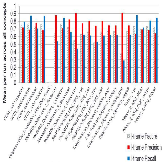
Fig. 12 2015: Temporal localization results by run
