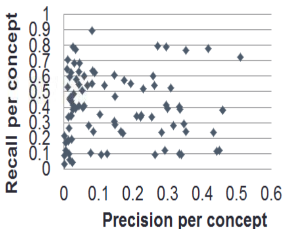
Fig. 13 2013: temporal precision and recall per concept for all teams
