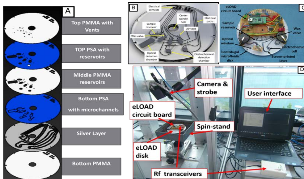
Figure 1: The electronically-enabled Lab-On-A-Disc (LoaD) platform with detection modules and heat-actuated wax valves.
