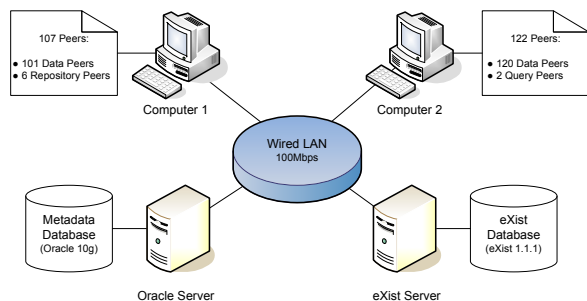
Figure 4. Network Configuration of the Chaotic P2P Network.
