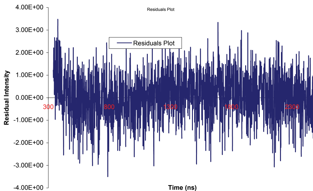
FIGURE C1: RESIDUAL DATA FOR DECAY OF 3 IN H 2 O, FIGURE 6.14(A).
