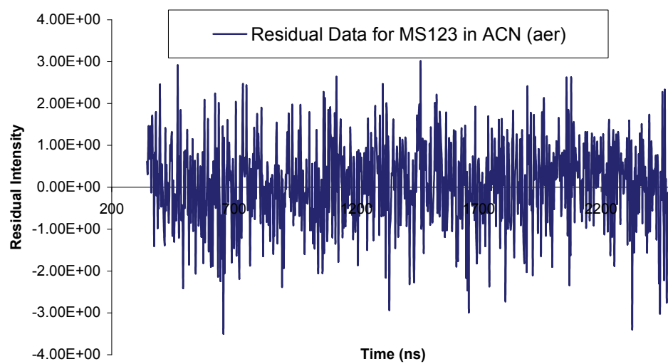
FIGURE C2: RESIDUAL DATA FOR DECAY OF 10 IN ACN (AER), AS SHOWN IN FIGURE 6.20.
