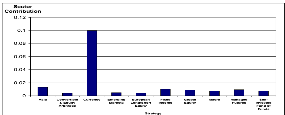
Fig. 9. Strategy Contribution, 3rd largest eigenvalue
