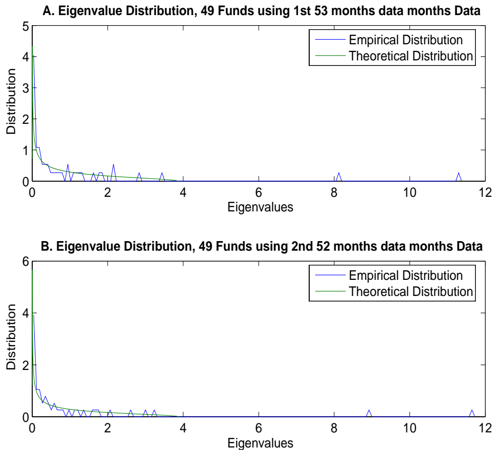
Fig. 2. Bootstrapped spectral distribution for consecutive periods.
