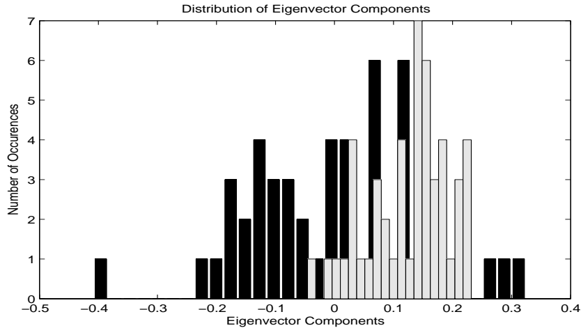
Fig. 3. Comparison of Eigenvector Components, largest Eigenvector (Grey), Eigenvector from the bulk (Black)
