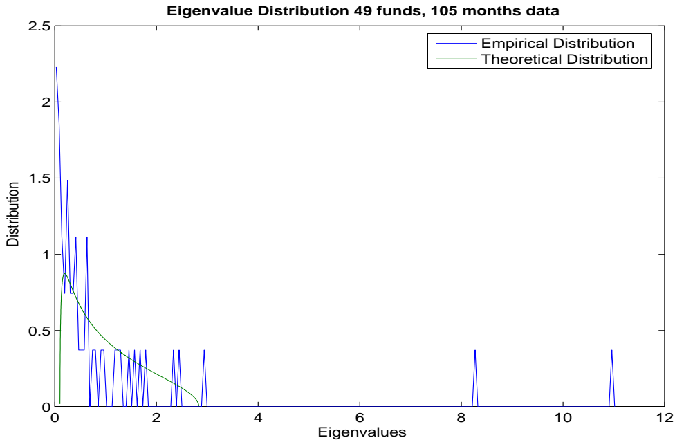
Fig. 1. Spectral Distribution for equally weighted Hedge Fund correlation matrix
