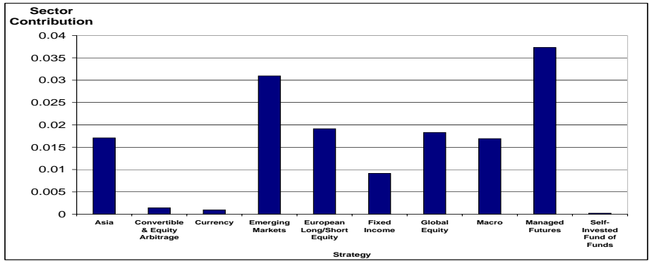
Fig. 7. Strategy Contribution, largest eigenvalue
