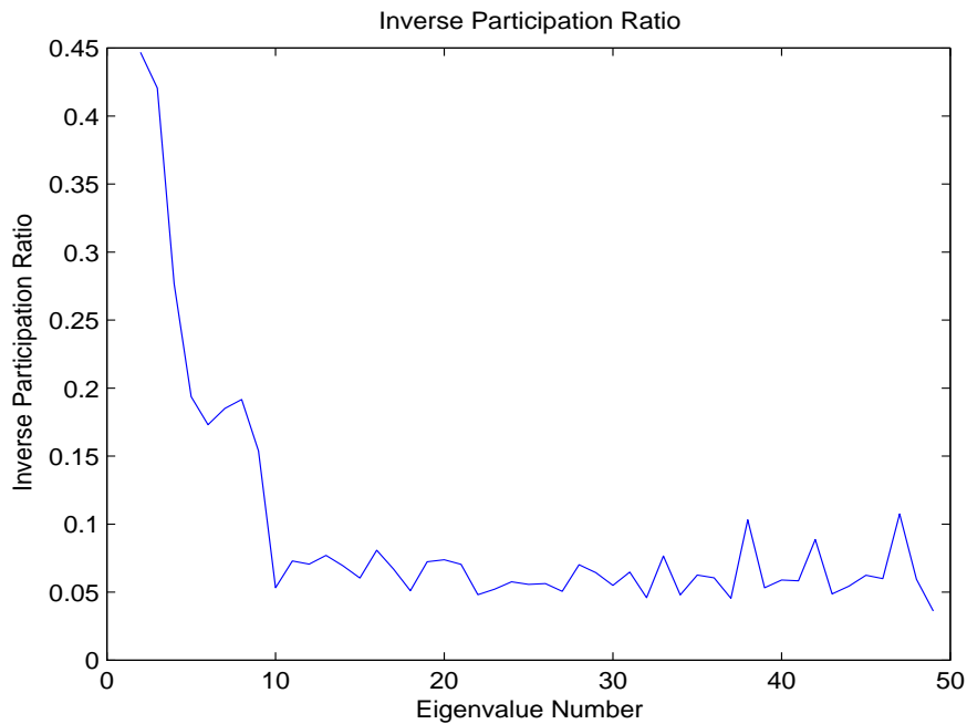
Fig. 10. Inverse Participation Ratio
