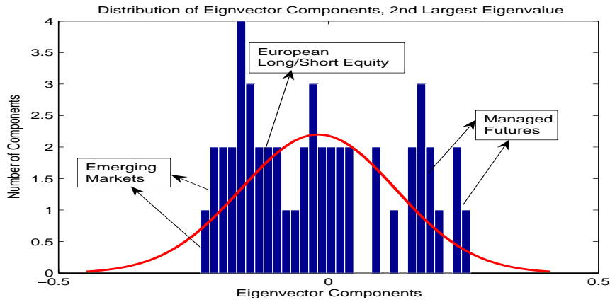
Fig. 5. Distribution of eigenvector components, largest remaining eigenvalue
