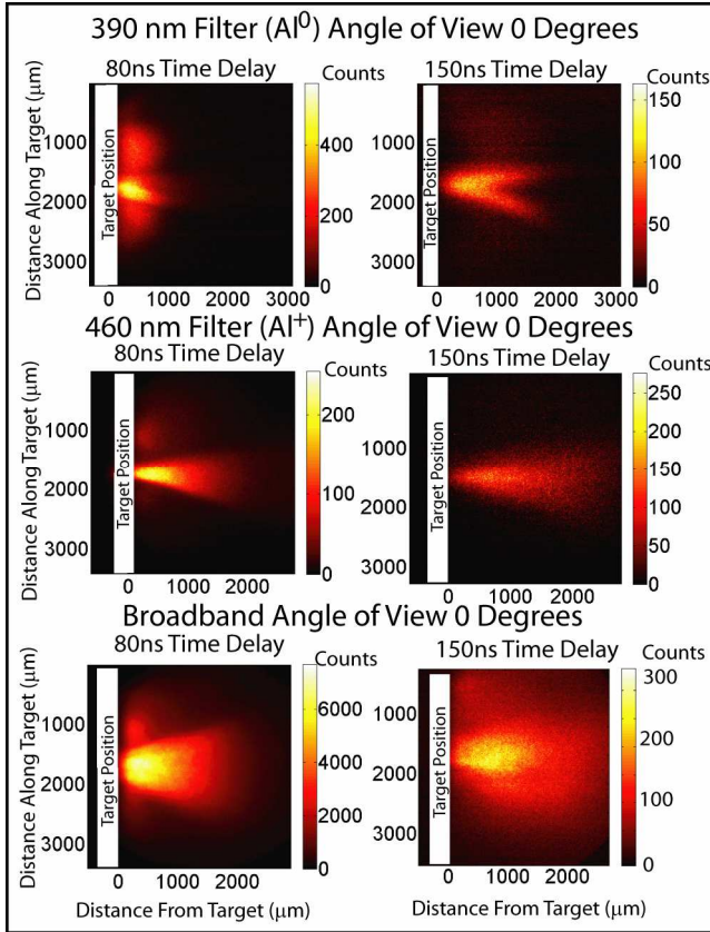
Figure 7: Comparison of emission from \text{Al}^0 , \text{Al}^+ and broadband imaging for a fixed viewing angle (0 Degrees) for two different delay times (80 ns – left panels and 150 ns – right panels).
