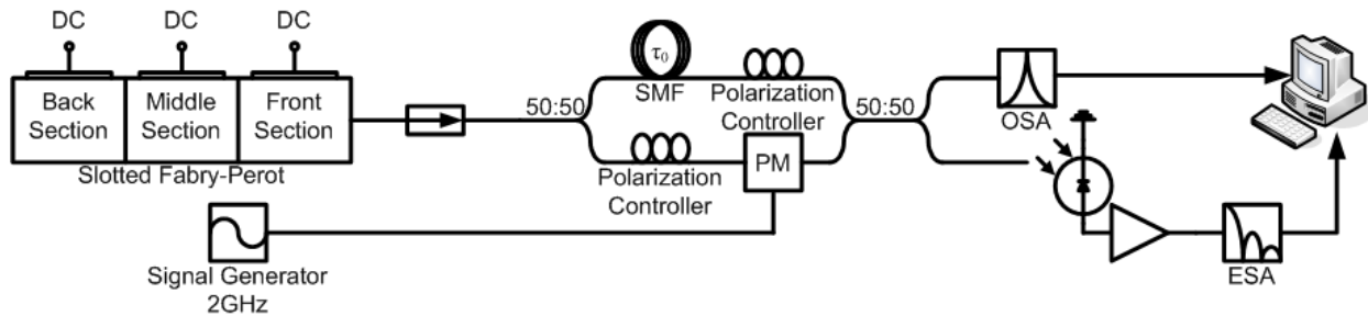
Fig. 1 Diagram of experimental setup
