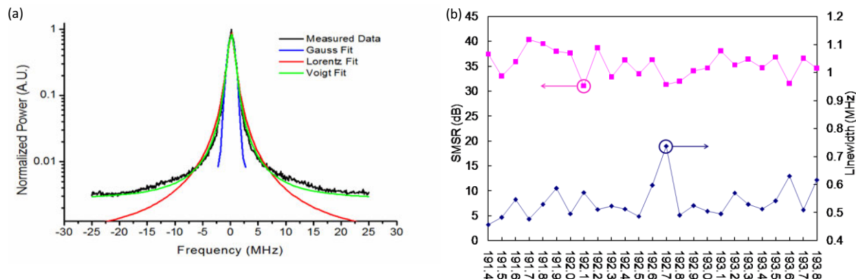
Fig. 3 (a) Lineshape of the SFP laser with Lorentzian (red line), Gaussian (blue line) and Voigt (green line) fitting. (b) Linewidth and SMSR.
