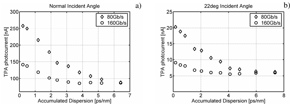
Fig. 2. CD monitoring of 80 Gb/s and 160 Gb/s data signal at (a) 1556 nm (normal incident angle) and (b) 1546 nm ( 22^\circ incident angle)
