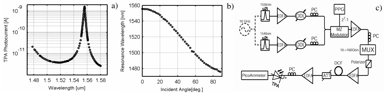
Fig. 1 (a) Cavity resonance characteristic, (b) Cavity resonance wavelength for varied incident angle, (c) Experimental Setup
