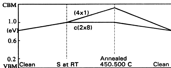
FIG. 7. Schematic illustration of the surface Fermi-level movements for sulfur deposition and annealing on the c (2×8) and (4×1) surfaces.
