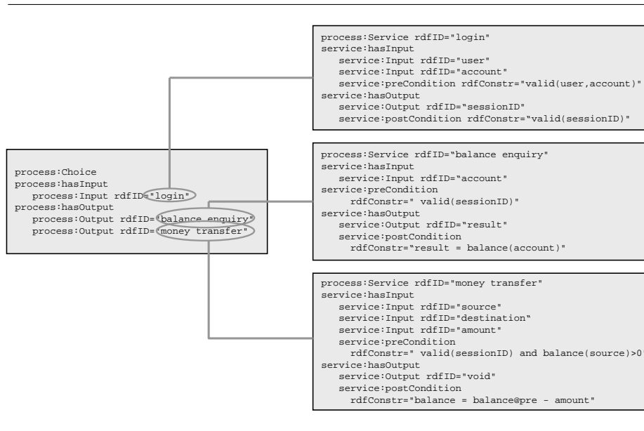
Fig. 4. WSPO Process and Service Model.
