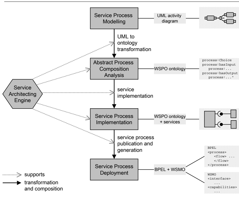
Fig. 1. Overview of the Ontology-based Service Architecture Technique.
