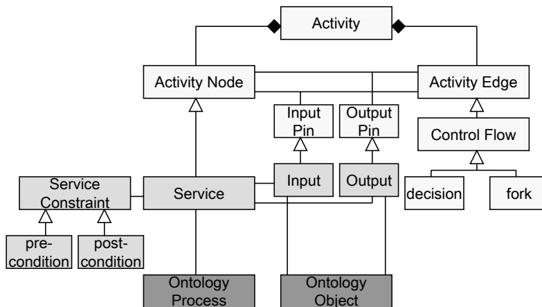
Fig. 2. UML Profile (Metamodel) for Semantic Service Process Modelling.
