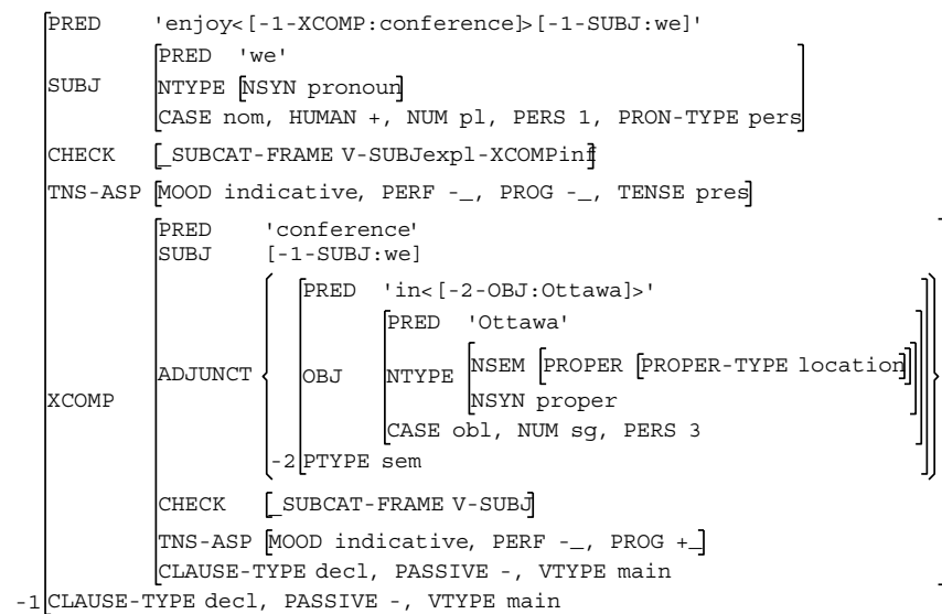
Figure 12: Tense and aspect in the extended DCU f-structures
