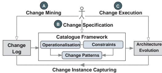
Figure 1: An Overview of Solution Framework.
