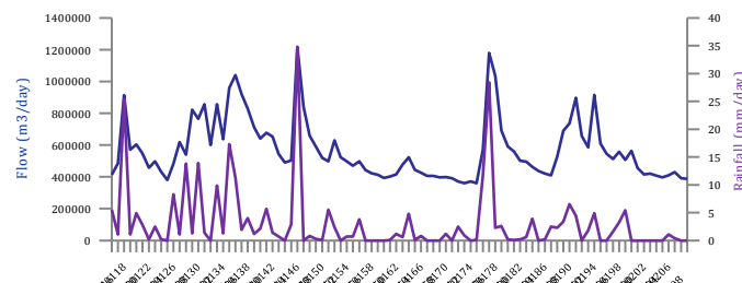
Figure 3 – Comparison between the flow levels through the WWTP (m 3 /day) to rainfall data (mm/day, collected from Met Eireann) at the tertiary WWTP
