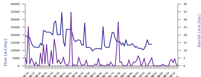
Figure 4 – Comparison between the flow levels through the WWTP (m 3 /day) to rainfall data (mm/day, collected from Met Eireann) at the secondary WWTP
