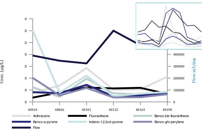
Figure 1 – PAH levels detected (µg L -1 ) and flow at the tertiary WWTP (m 3 /day)
