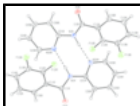
Fig. 1. A view of the hydrogen bonded dimeric unit in (I) with the atomic numbering scheme for the two independent molecules A and B. Displacement ellipsoids are drawn at the 30% probability level.
