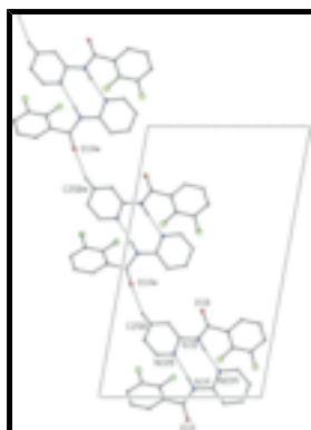
Fig. 3. A view of the primary interactions in the crystal structure of (I) with H atoms not involved in hydrogen bonding removed for clarity. Molecules in the hydrogen bonded dimer with suffixes A and B are linked to symmetry related dimers at positions * and # via C—H...O interactions.
