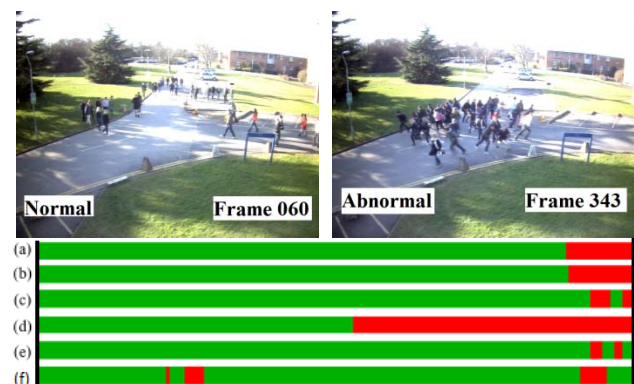
Figure 4: Crowd escape behavior detection for view 2 in the second scenario of PETS2009 dataset. (a) Ground truth, (b) result of the proposed method, (c) result of BM, (d) result of FF, (e) result of CI and (f) result of SF.
