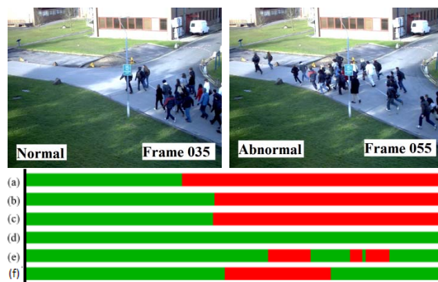
Figure 3: Crowd escape behavior detection for view 1 in the first scenario of PETS2009 dataset. (a) Ground truth, (b) result of the proposed method, (c) result of BM, (d) result of FF, (e) result of CI and (f) result of SF.
