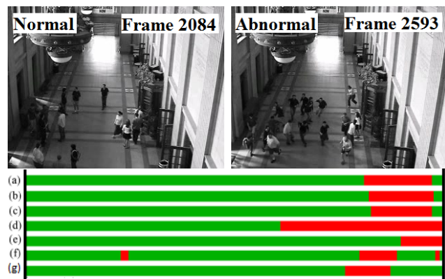
Figure 2: Crowd escape behavior detection for scenario 6 in the UMN dataset. (a) Ground truth, (b) result of the proposed method, (c) result of BM, (d) result of FF, (e) result of CI, (f) result of SF, and (g) result of SRC.
