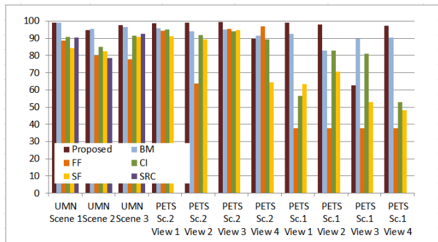
Figure 5: Accuracy comparisons of the proposed method with BM, FF, CI, SF and SRC on all scenarios for UMN and PETS2009 datasets.
