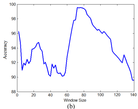
Figure 6: The effect of window size on accuracy. (a) Accuracy performances with differing window size in the UMN dataset. (b) Accuracy performances with differing window size in the PETS2009 dataset for the second scenario.
