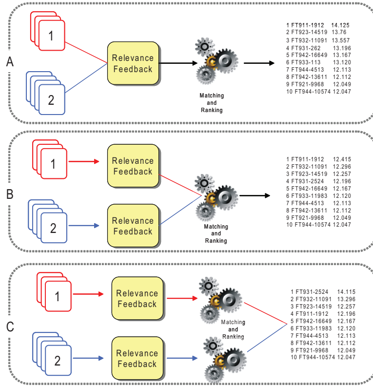
Figure 2. Combining relevance information, the 3 choices
