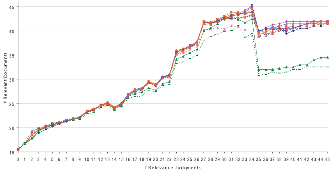
Figure 6. Comparison of collaborative relevance feedback techniques and baseline division of labour system across all topics
