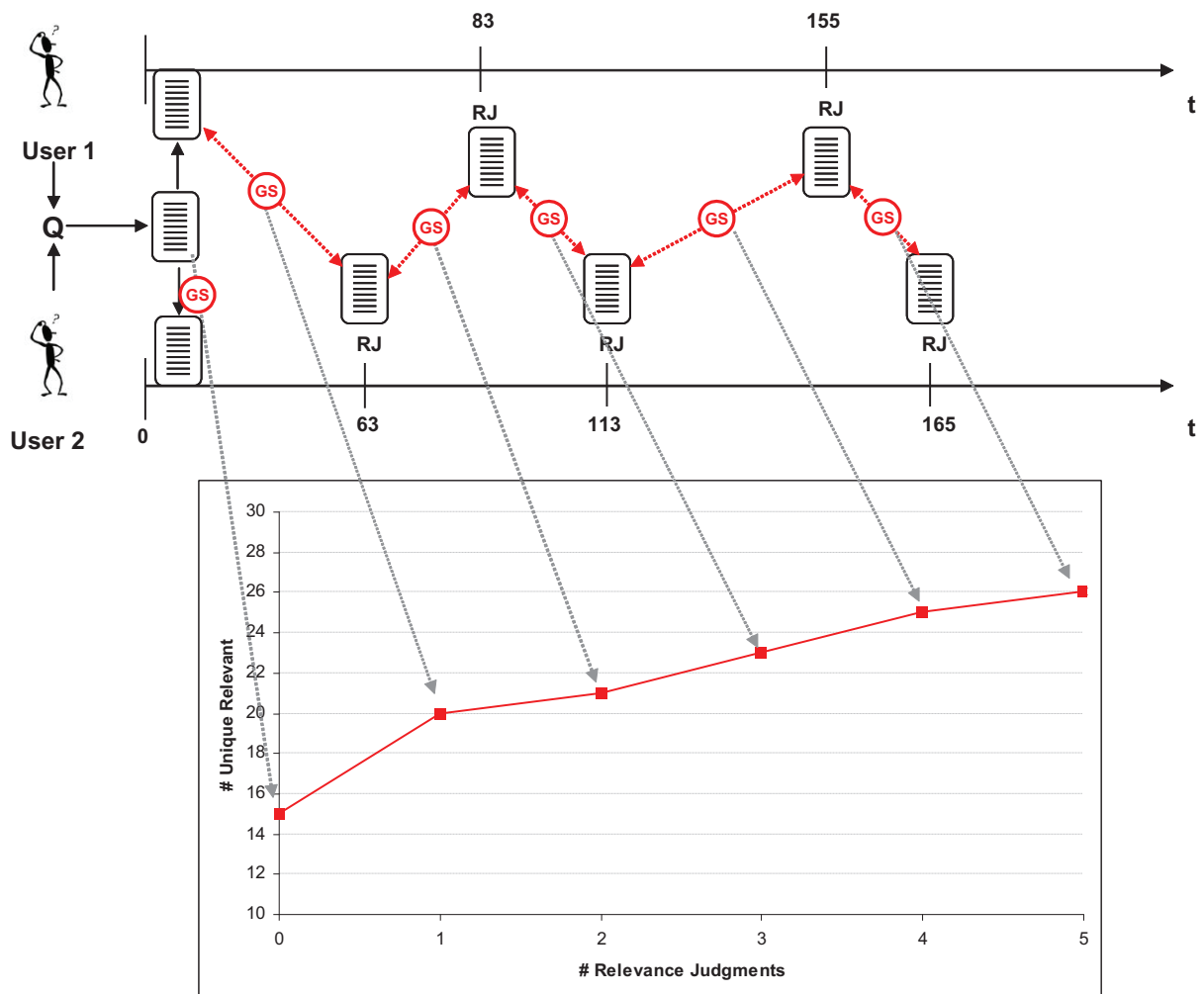
Figure 5. Measurement granularity used in experiments
