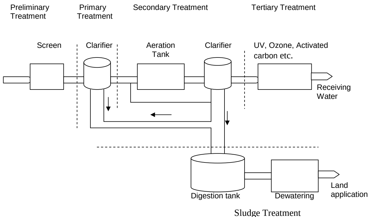
Figure 1.3.1 Schematic of wastewater treatment (Adapted from Swords WWTP schematic).
