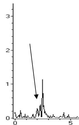
d) Trimethoprim: Influent + 4 µg/L standard
