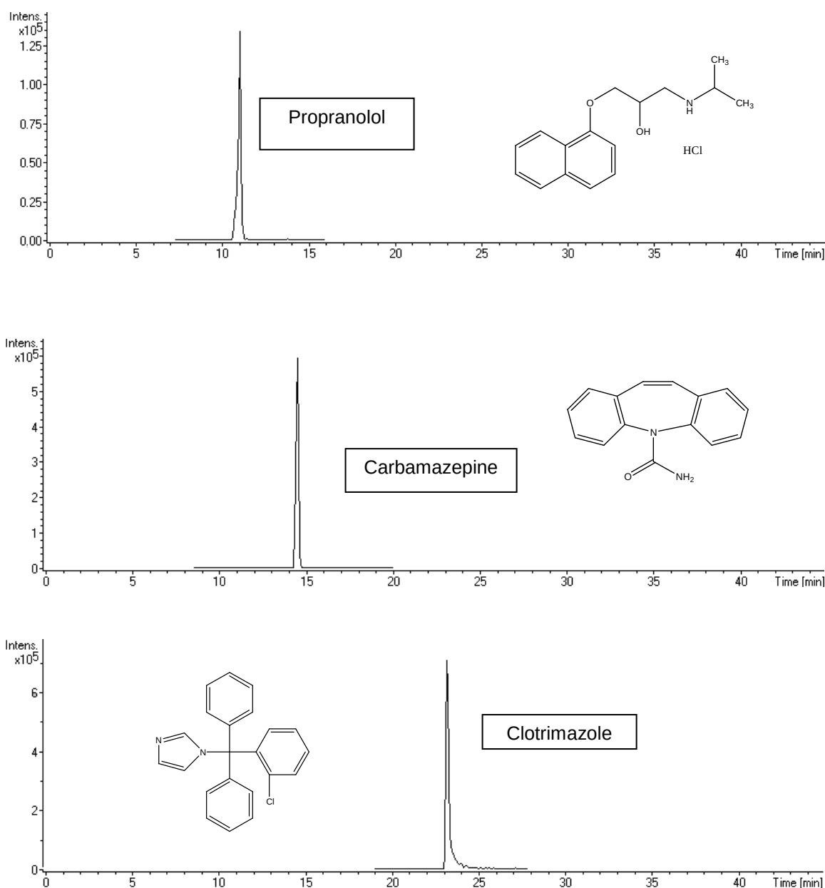
Figure 3.1.2b (continued). Chromatograms of a 5µg/mL standard in influent matrix analysed using positive ionisation.
