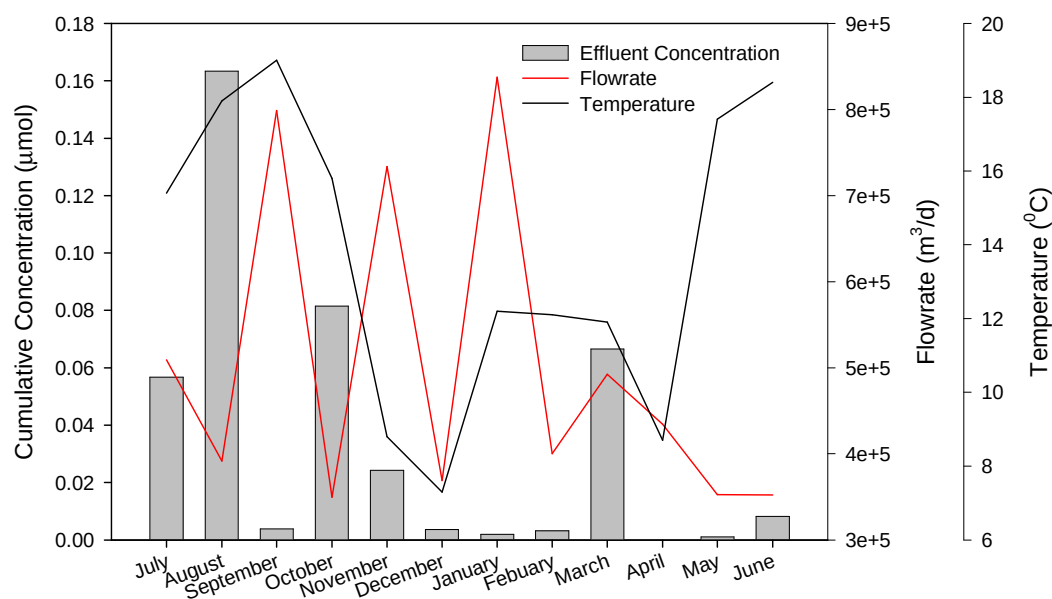
Figure 4.4.2 Cumulative concentration of pharmaceuticals in effluent at Ringsend WWTP and daily temperature and flowrates (July 2007 – June 2008)
