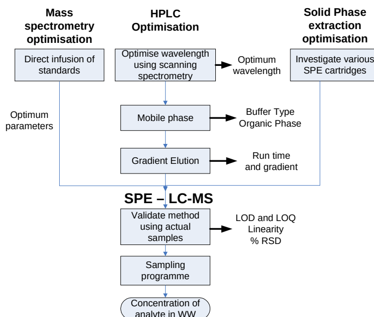
Figure 2.5.2 Overview of SPE-LC-MS/MS method development and validation
