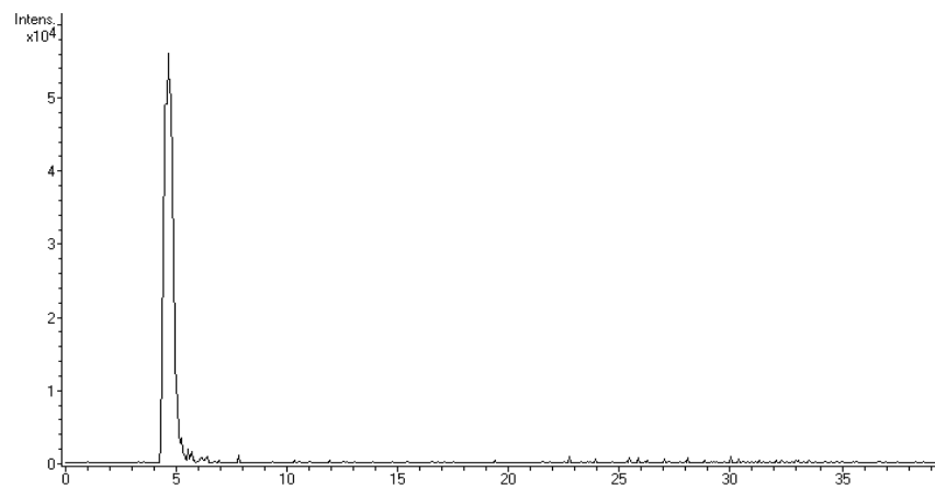
a) Trimethoprim standard
