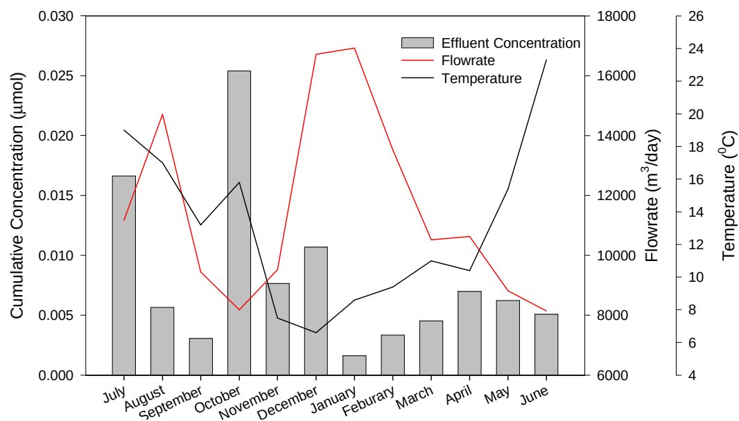
Figure 4.4.1 Cumulative concentration of pharmaceuticals in effluent at Leixlip WWTP and daily temperature and flowrates (July 2007 – June 2008)
