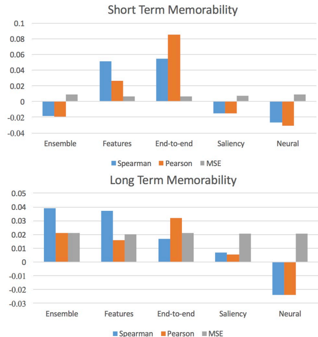
Figure 1: Performance for memorability classification
