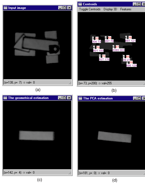
Figure 12: Recognition results when the system is applied to a scene containing clutter and occlusion. (a) The input image. (b) The resulting image data. (c) The topmost recognized region. (d) The pose estimation for the topmost object.
