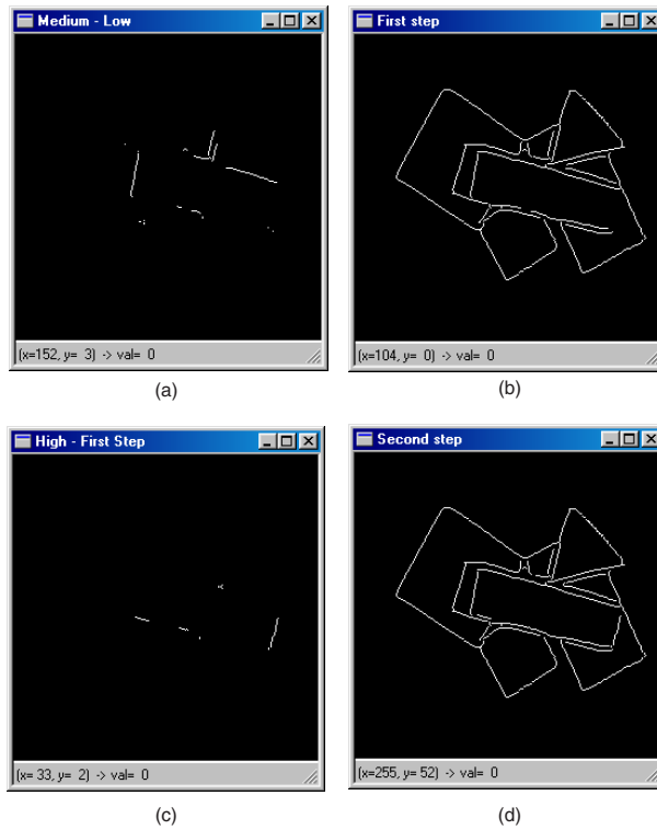
Figure 6: The edge reconstruction process for images illustrated in Fig. 5. (a) Difference between the medium and lowest resolution images. (b) The resulting image after first iteration. (c) Difference between (b) and the highest resolution image. (d) The output image.
