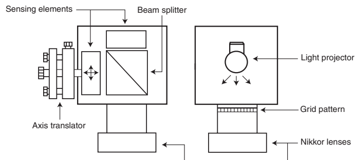
Figure 3: The bifocal range sensor.
