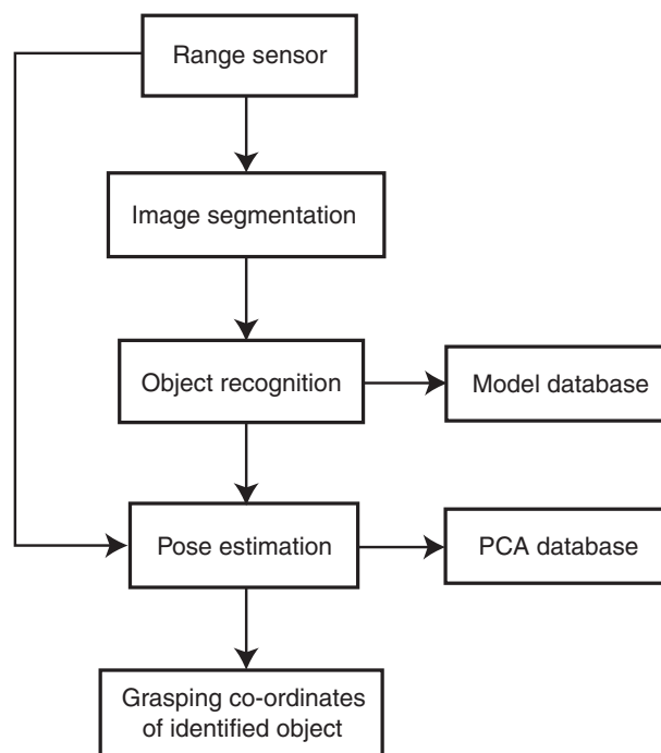
Figure 1: Overall system architecture.
