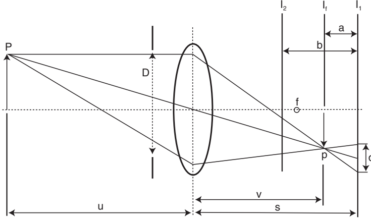
Figure 2: The image formation process. Depth is determined by measuring the relative level of blurring.
