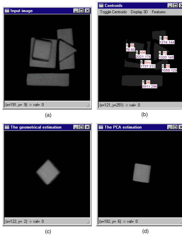
Figure 11: Recognition results when the system is applied to a scene containing clutter. (a) Input image. (b) The resulting image data (the first figure defines the rank of the region with respect to area, the second is the region's elevation and the last two represent the region's area and perimeter). (c) The topmost recognised region. (d) The pose estimation for the topmost object.
