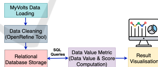
Figure 2: An Overview of the Automatic Metric-based Approach.
