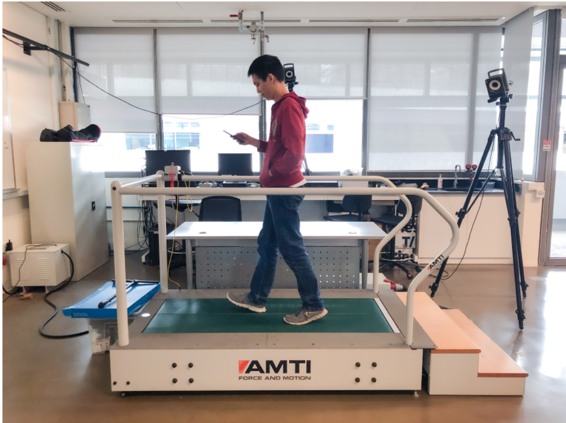
Fig. 8. Experimental setup for the treadmill conditions
