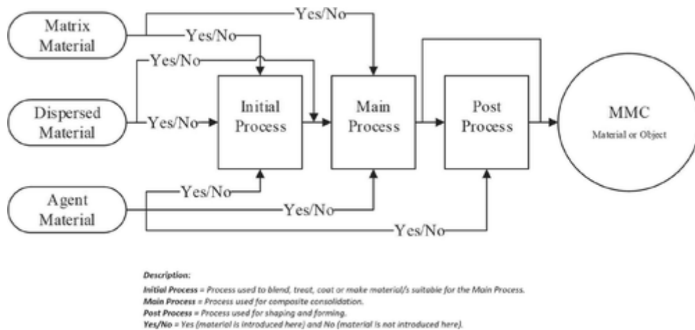
FIGURE 2 Overview flowchart of the processing steps involved during production of a MMC
