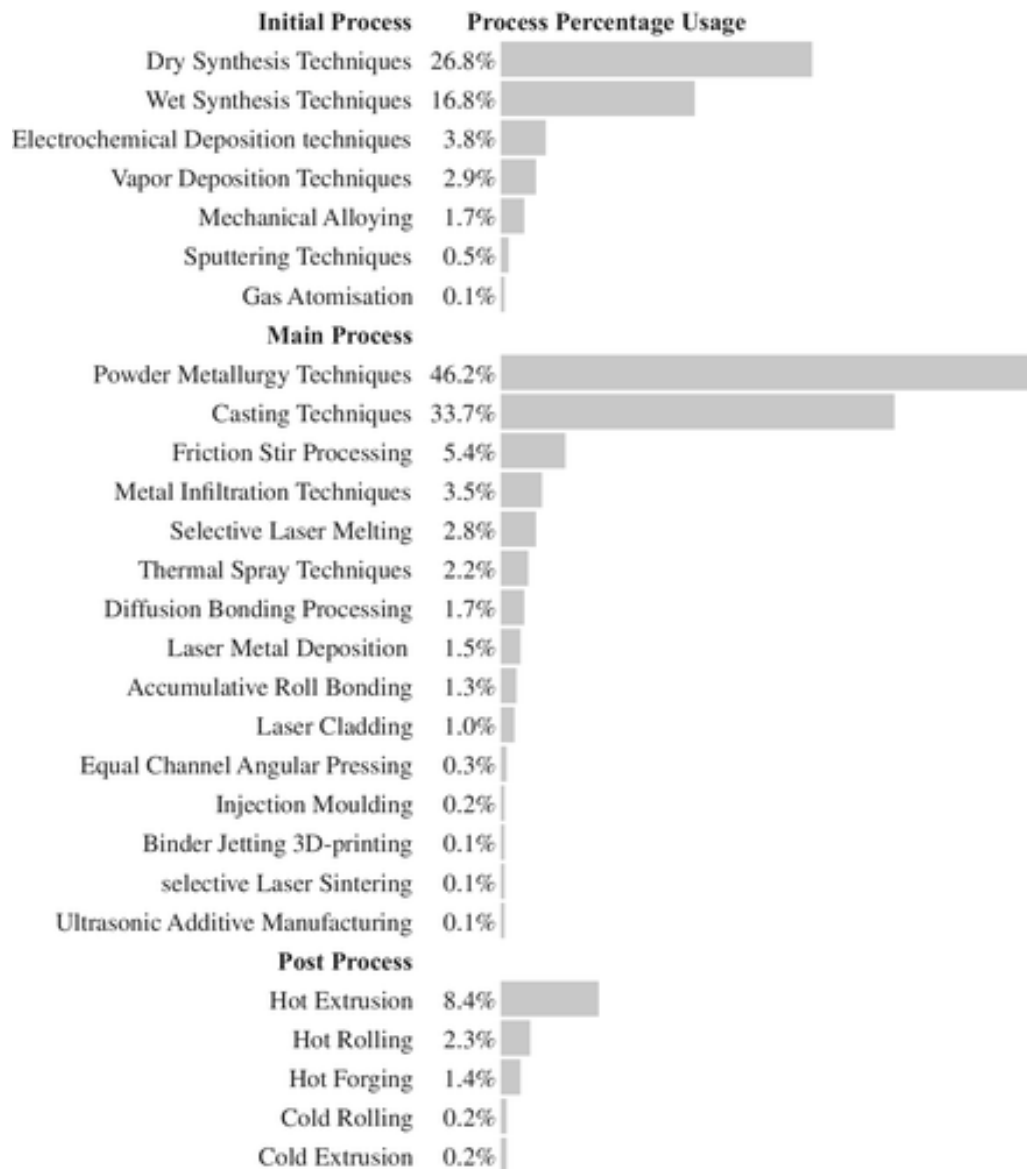
FIGURE 3 Extent of process utilization for MMC production research and development
