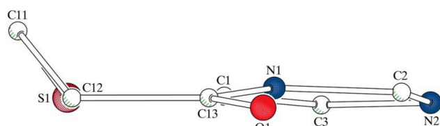
Figure 2 An edge-on view of the [6–5] fused-ring system in (Ia), highlighting the envelope conformation.
