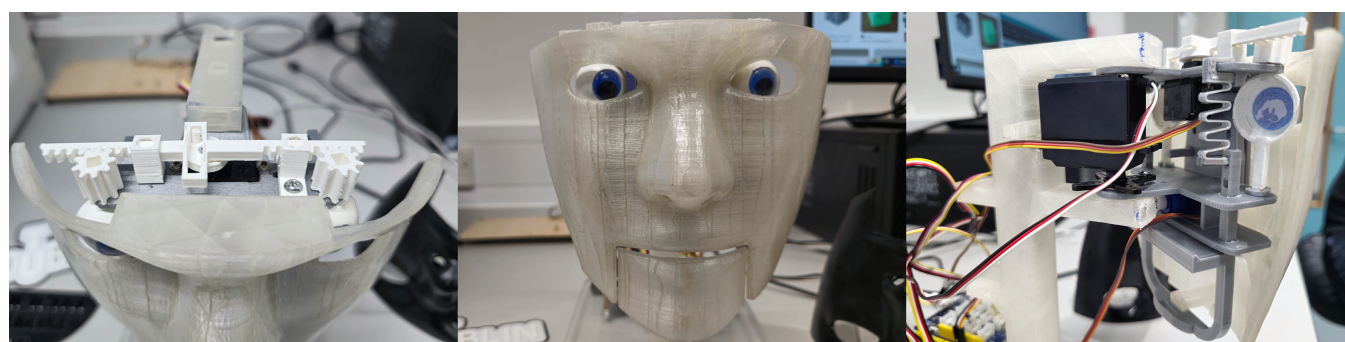
Figure 1: AI talking mask (centre). Eye movement mechanism (left). Jaw mechanism (right).
