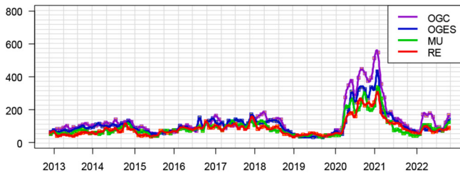
Fig. 7. Aggregate and sector-wise connectedness.
