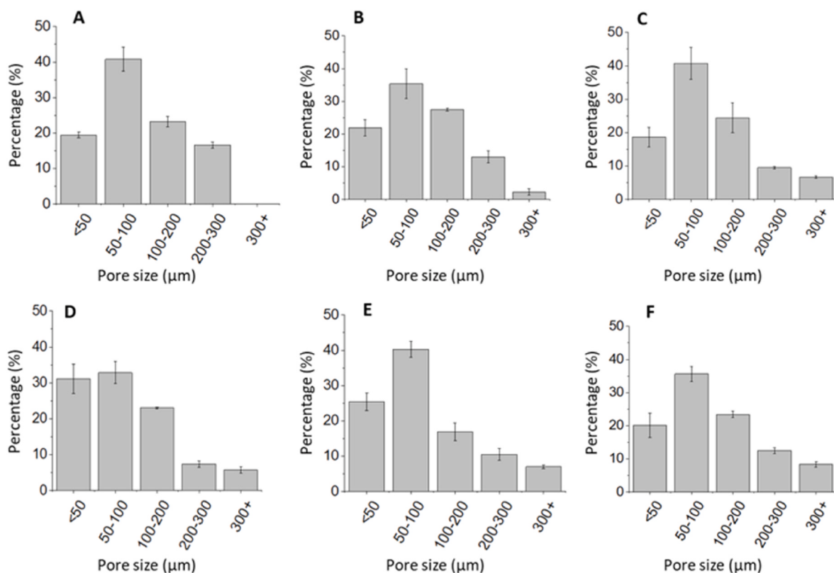
Fig. 8. Pore size distribution over time for 100CSH formulation analysed using Micro-CT CT-An software. A: Initial pore size distribution of the cement. B: Pore size distribution at Day 3. C: Pore size distribution at Day 7. D: Pore size distribution at Day 14. E: Pore size distribution at Day 21. F: Pore size distribution at Day 28.
