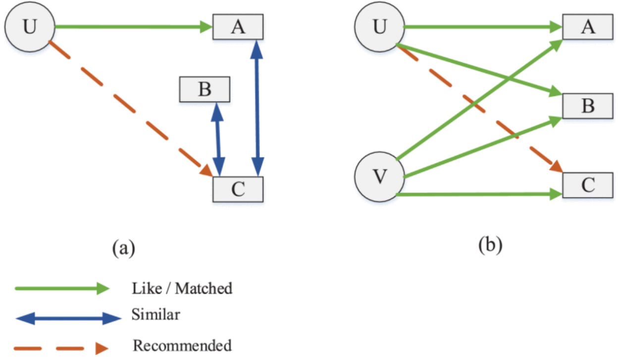
Fig. 1. (a) Content filtering. (b) CF.
