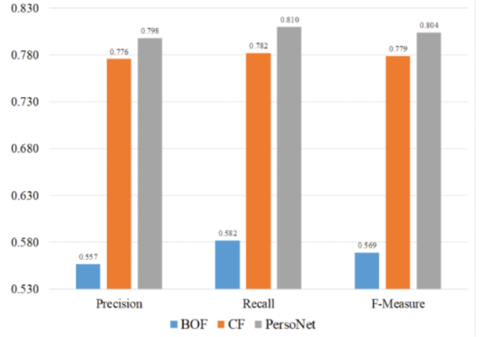
Fig. 7. Systems evaluation with message-exchange-based similarity
