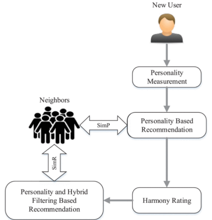
Fig. 2. PersoNet's system design.
