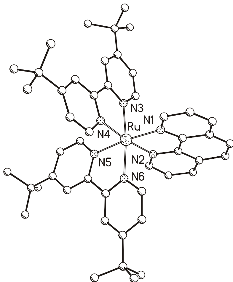
Figure S1. Molecular structure of (tbbpy)_2Ru(phen) , 2 , Anions and hydrogen atoms omitted (Ru-N bond length in Å, angles in °, Ru-N1 2.061(5), Ru-N2 2.056(5), Ru-N3 2.053(4), Ru-N4 2.055(4), Ru-N5 2.060(4), Ru-N6 2.074(4), N1-Ru-N2 79.9(2), N3-Ru-N4 77.88(16), N5-Ru-N6 78.99(16))
