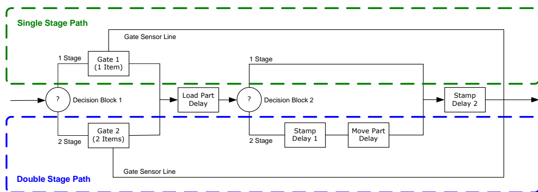
Figure 4.10: Simplified press hierarchical block diagram showing paths for single and double stage pressing capability
