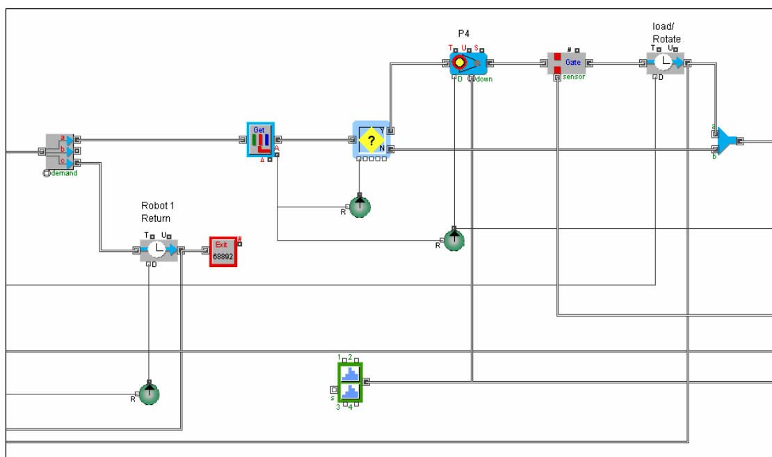
Figure A.4: Robot 1 return dummy path and first Press 4 stage.
