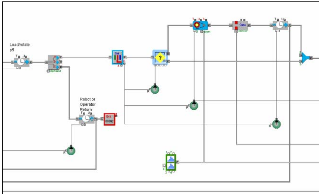
Figure A.7: Load Press 5 and first pressing stage.
